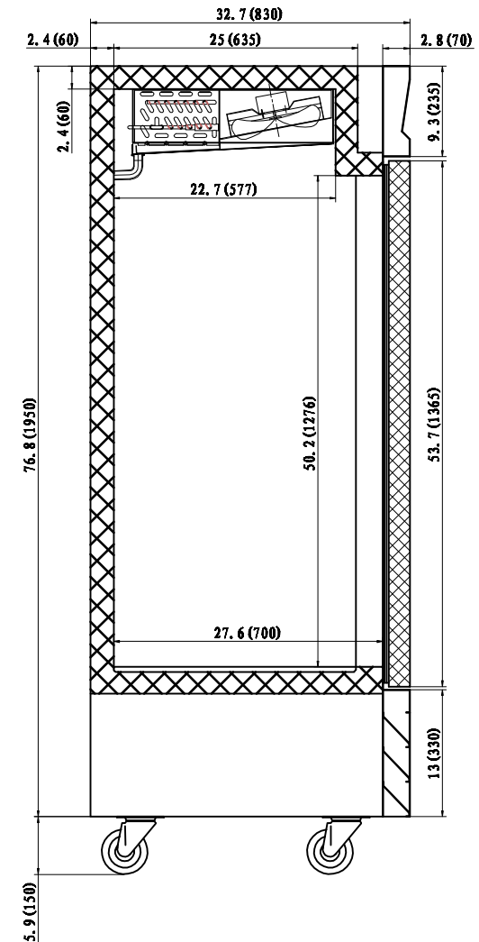
Dimensional Drawing VP3R-HC / VP3FDV-HC
